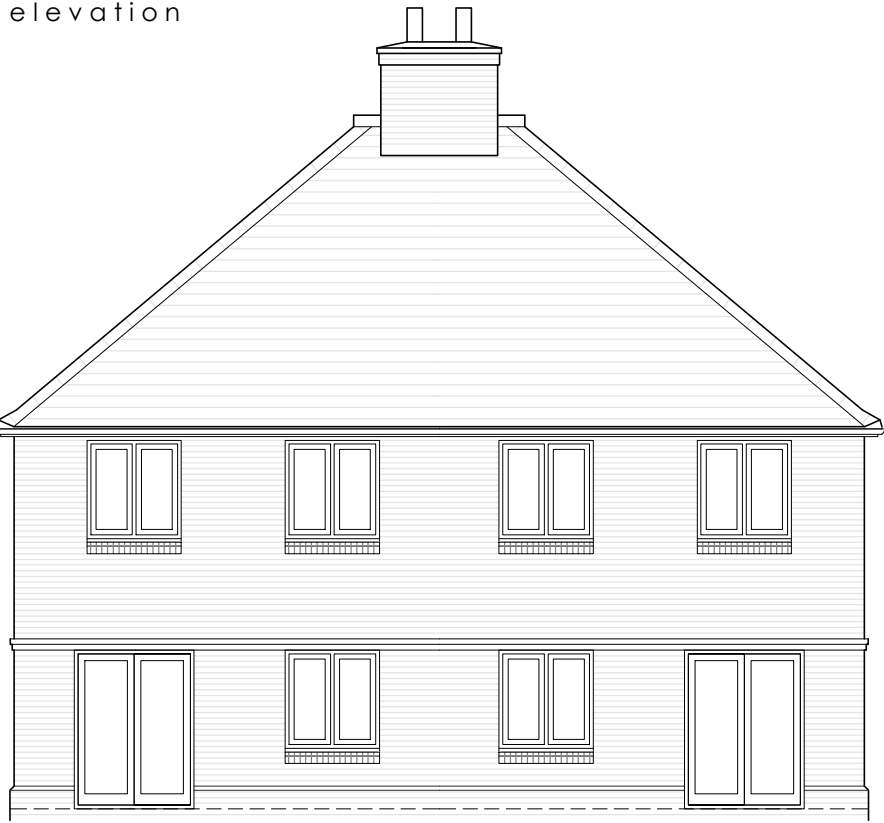
REAR elevation
