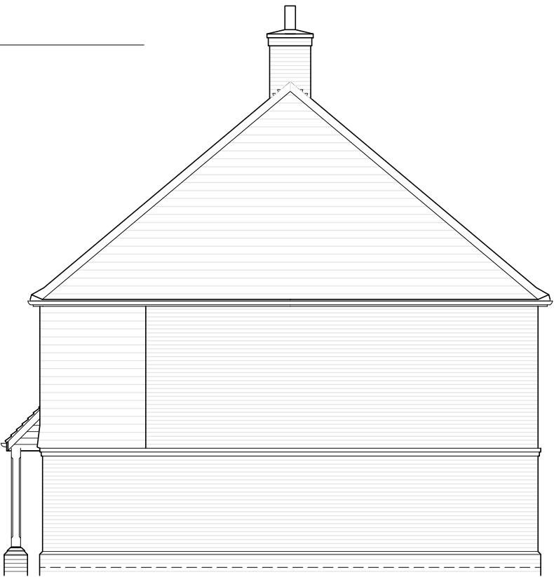
SIDE elevation
