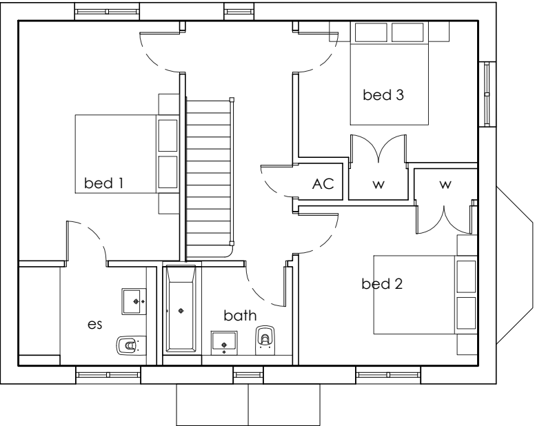
FIRST plan
