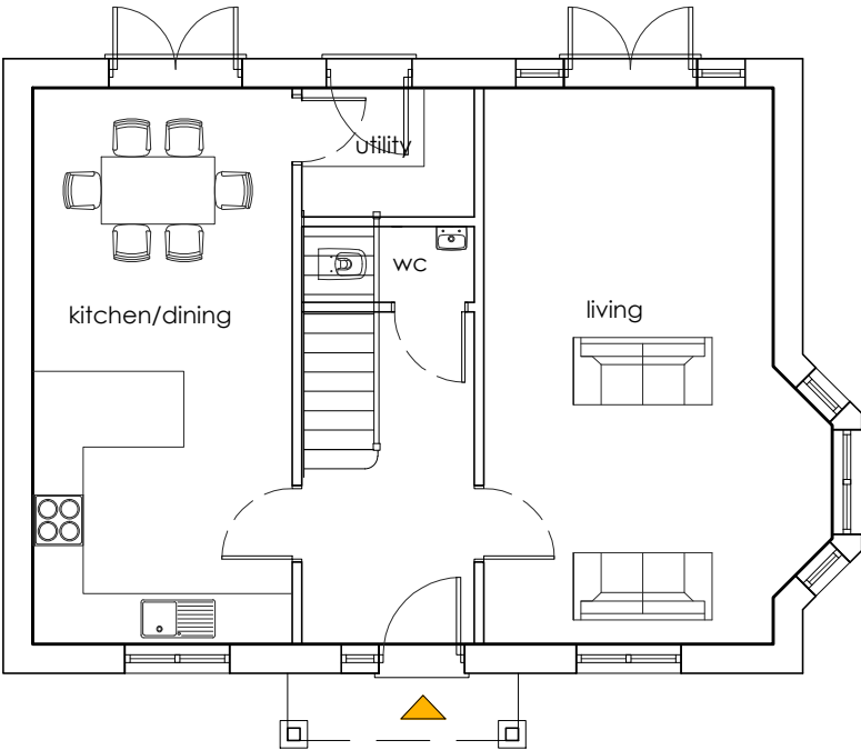
GROUND plan
