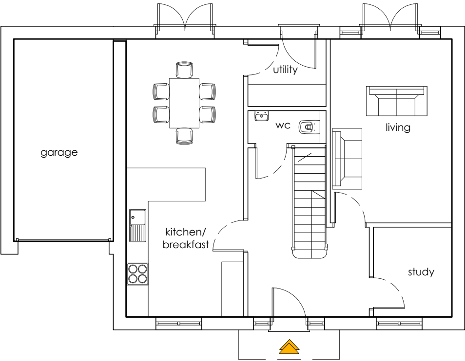
GROUND plan
