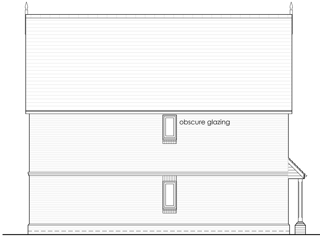
SIDE elevation
