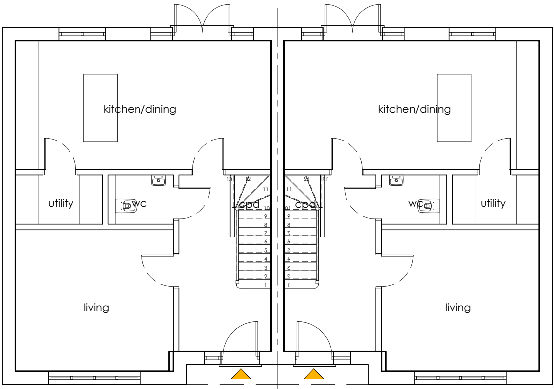
GROUND plan
