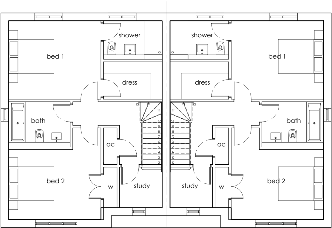
FIRST plan
