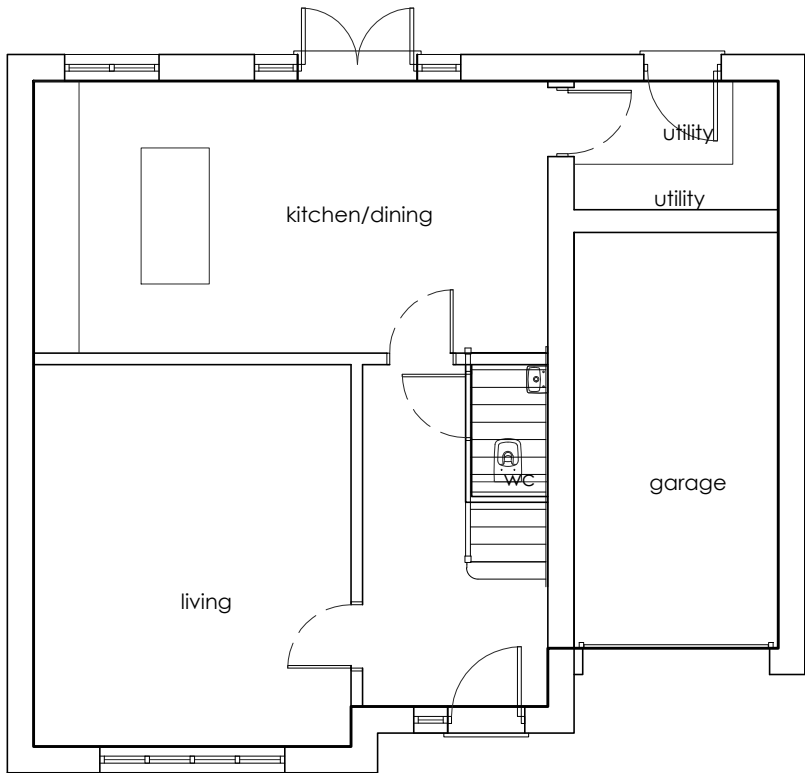
GROUND plan
