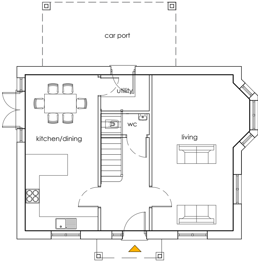
GROUND plan
