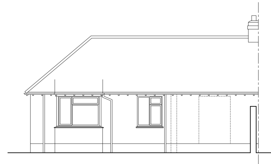
Existing South Elevation (rear) 1:100 @ A3
