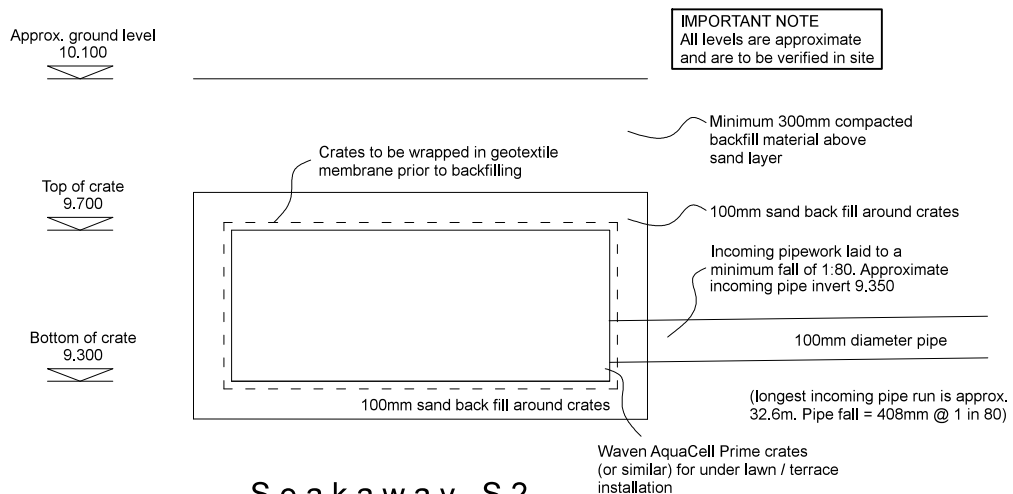
Soakaway S2 Detail B
