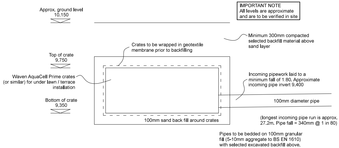
Soakaway S1 Detail A
