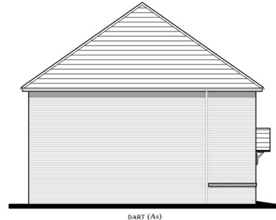
Side Elevation
