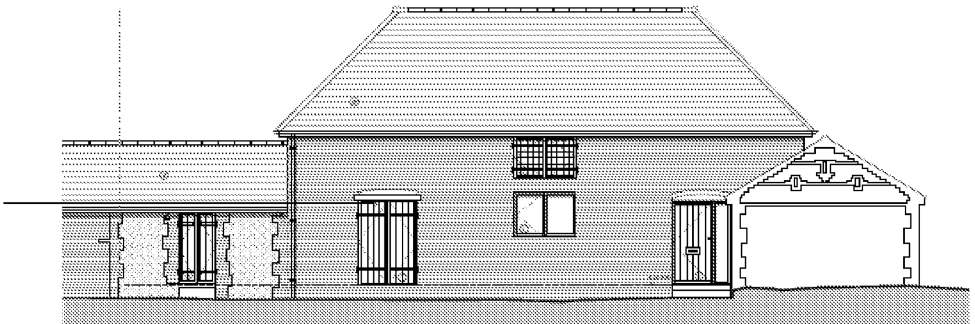
Proposed South East Elevation (B)
