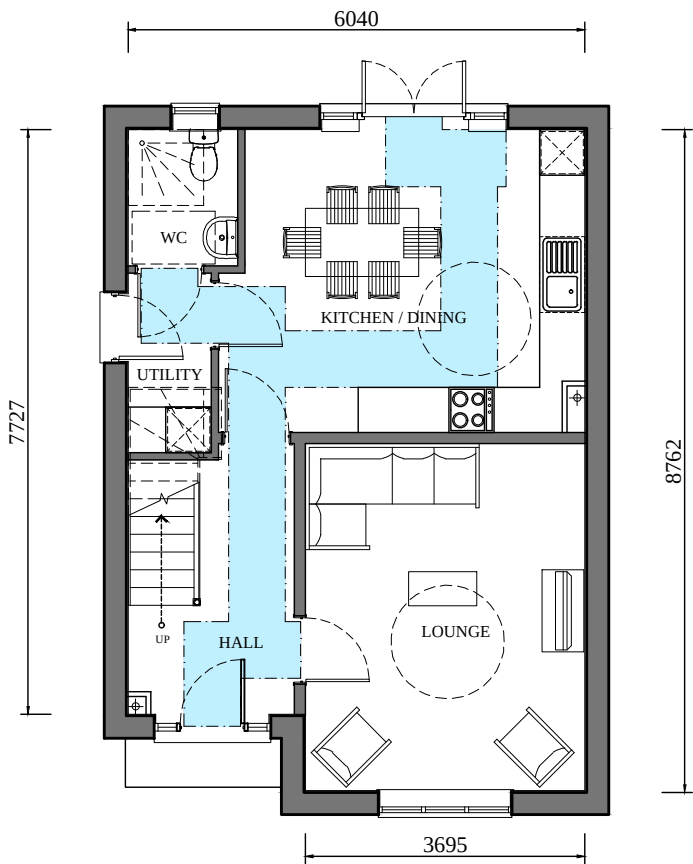
GROUND FLOOR (1:100)
