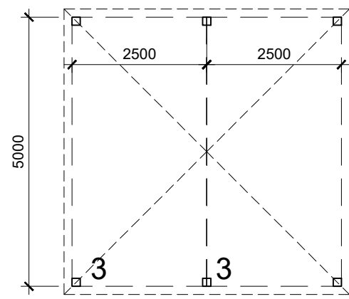
Car Barn 3 - Proposed Plan
