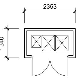
Pump House - Proposed Plan
