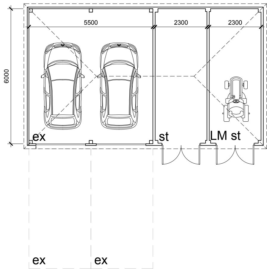
Car Barn 2 - Proposed Plan
