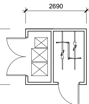
Barn 3 Bin & Cycle Store - Proposed Plan
