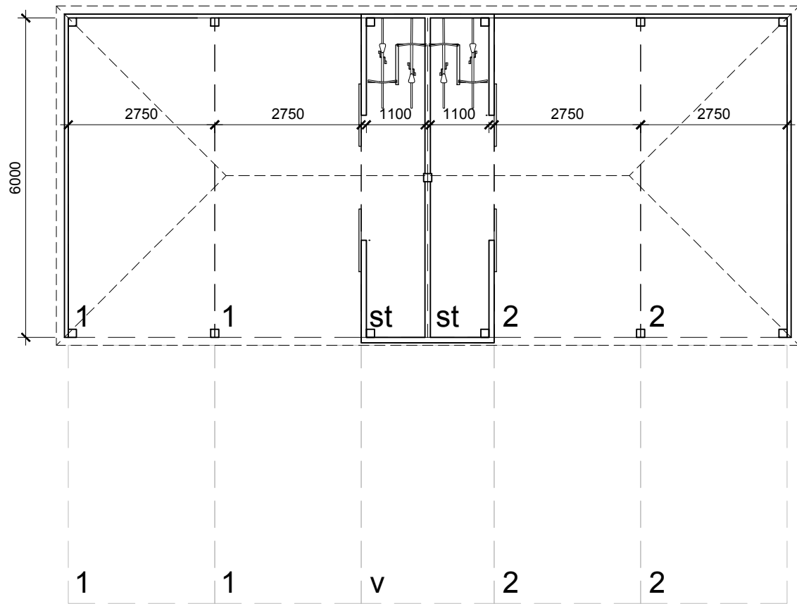
Car Barn 1 - Proposed Plan
