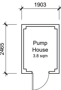
Pump House - Proposed Plan
