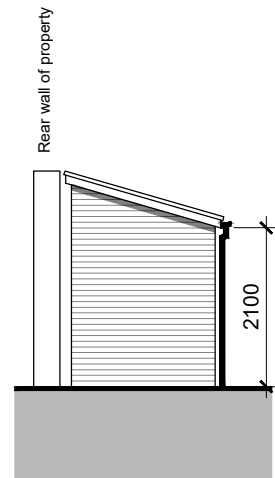
Rear Elevation
