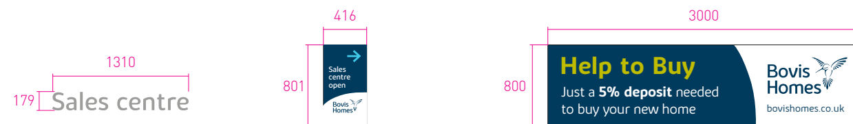
ITEM J - ACM CUT LETTERS DEPTH: 15MM
