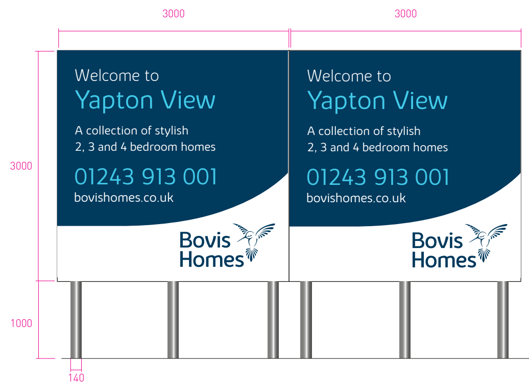
ITEM A - MAIN TOTEM V-BOARD DEPTH:163MM
