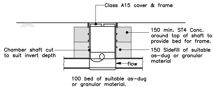
250mm \varnothing Inspection Chamber Section
