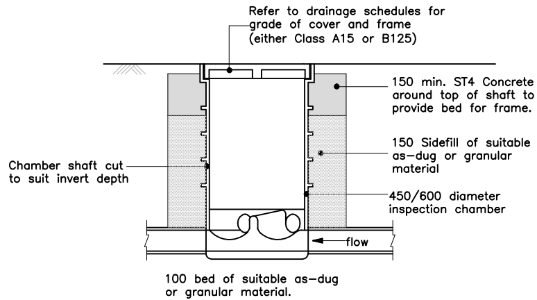
600 & 450mm \varnothing Inspection Chambers Section
