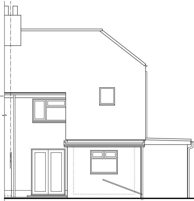
South Elevation
