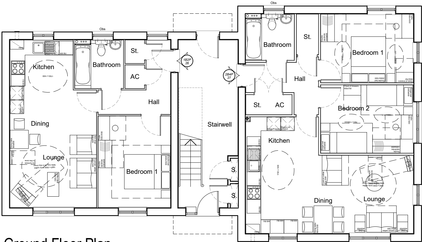
Ground Floor Plan *Obs - Obscured Glass
