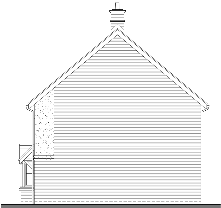
Side Elevation
