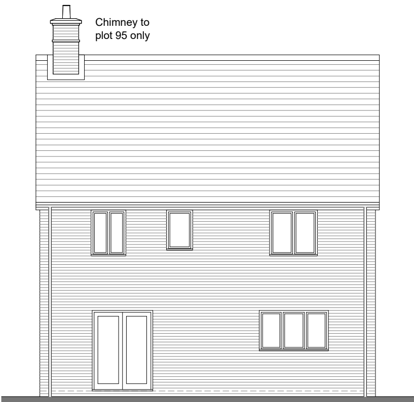
Rear Elevation
