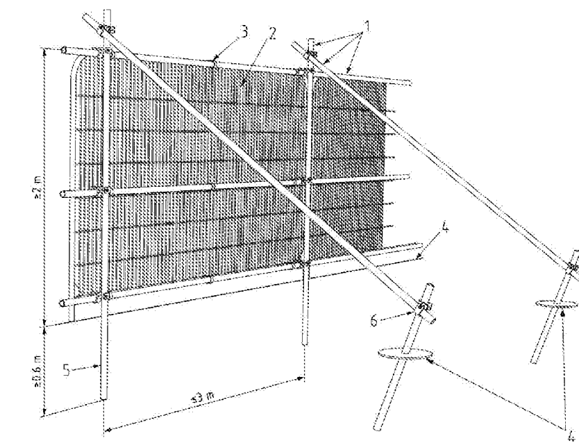
BS:5837:2012 Figure 2 Default specification for protective barrier
