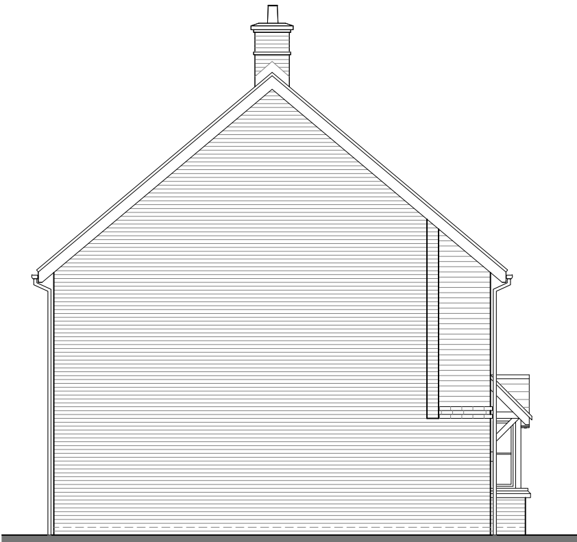
Side Elevation
