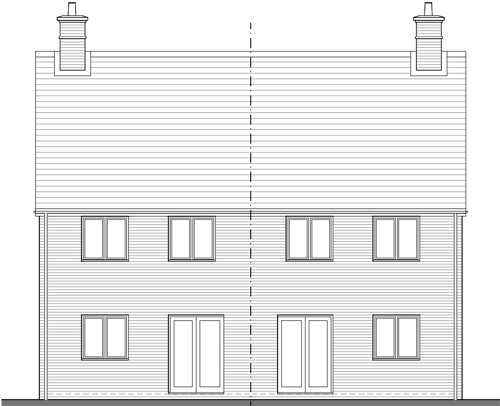
Rear Elevation
