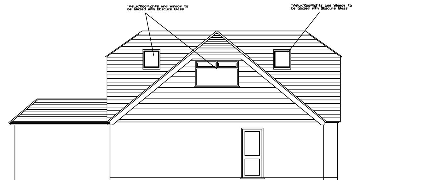
Proposed West Elevation Proposed Garage Side Elevation
