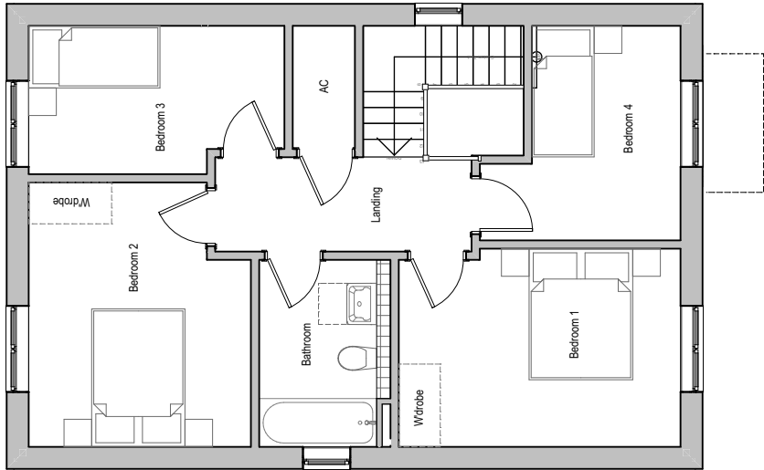
Proposed First Floor Plan 1:100 @ A2
