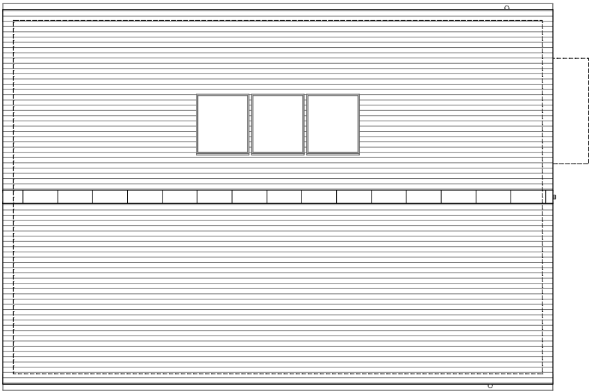
Proposed Roof Plan 1:100 @ A2
