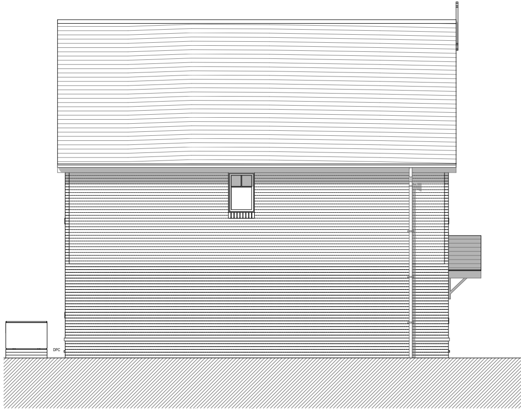
Proposed Side Elevation 1:100 @ A2
