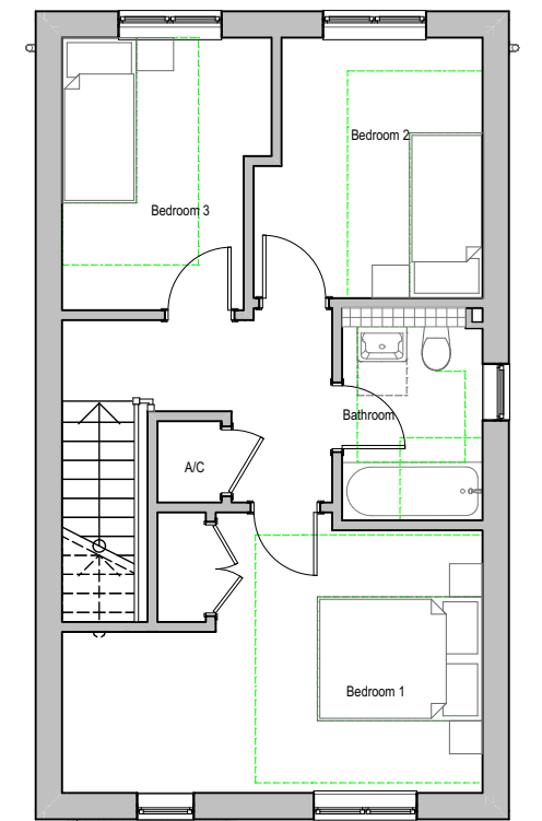
Proposed First Floor Plan 1:100 @ A2
