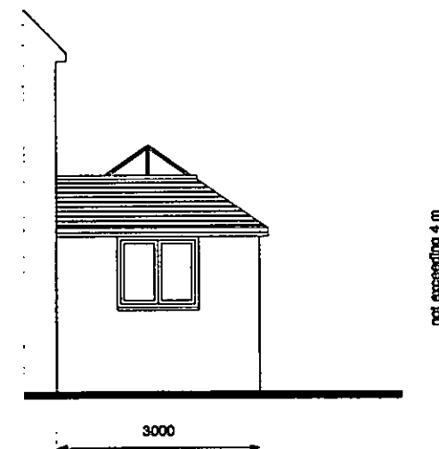
Proposed North West (Side) Elevation at 1:100 scale
