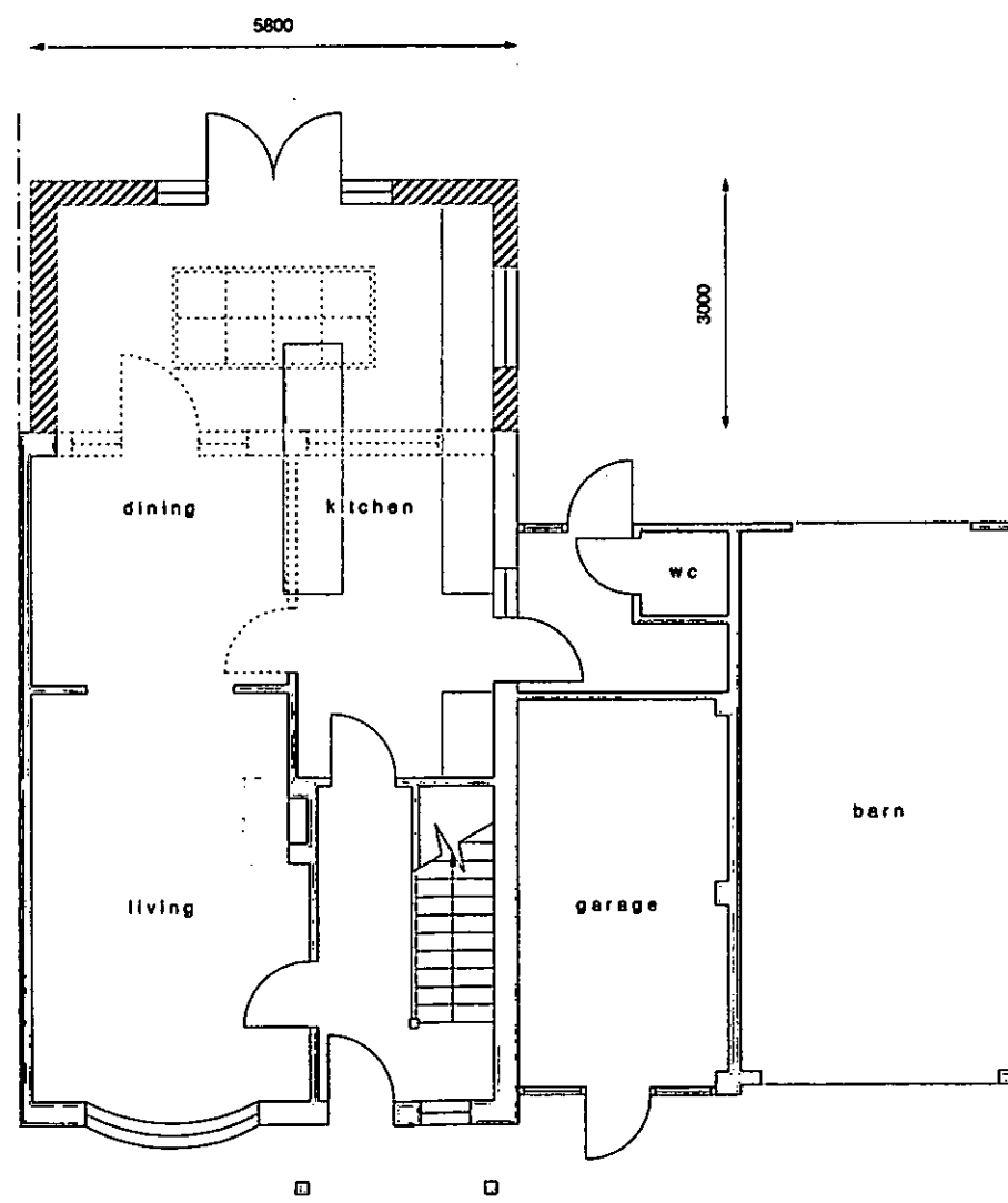
Proposed Ground Floor Plan at 1:100 scale
