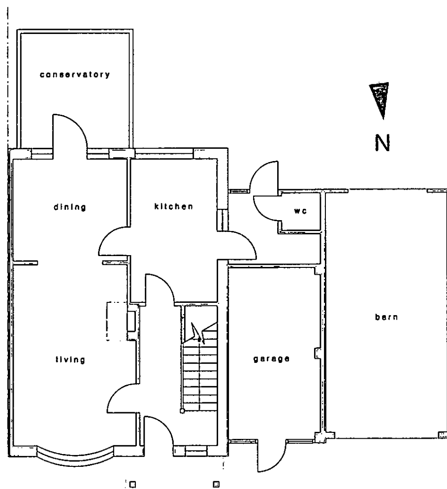
Existing Ground Floor Plan at 1:100 scale
