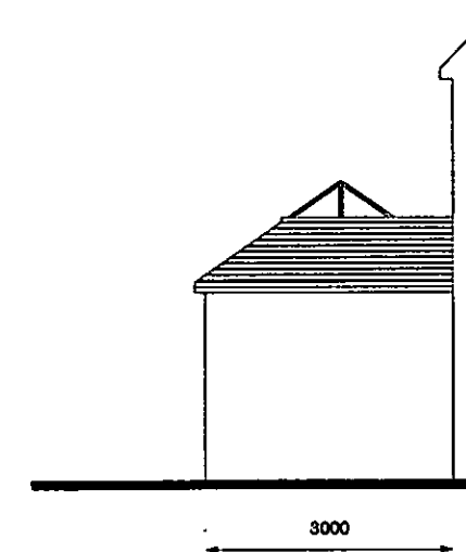
Proposed South East (Side) Elevation at 1:100 scale
