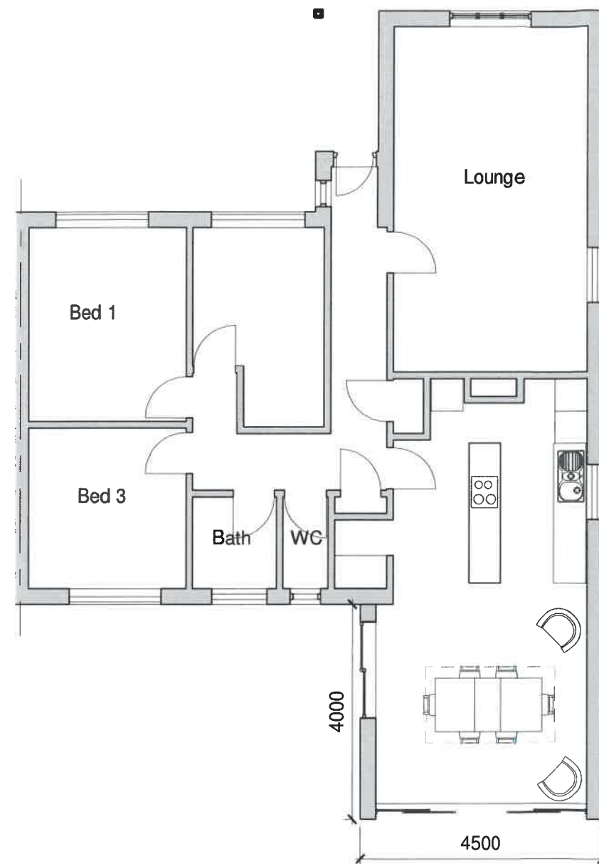
Proposed Ground Floor 1 : 100
