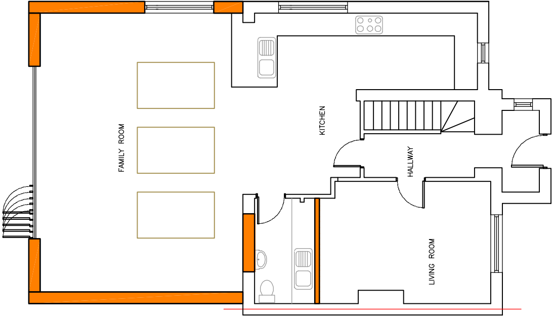
PROPOSED GROUND FLOOR PLAN 1:100
