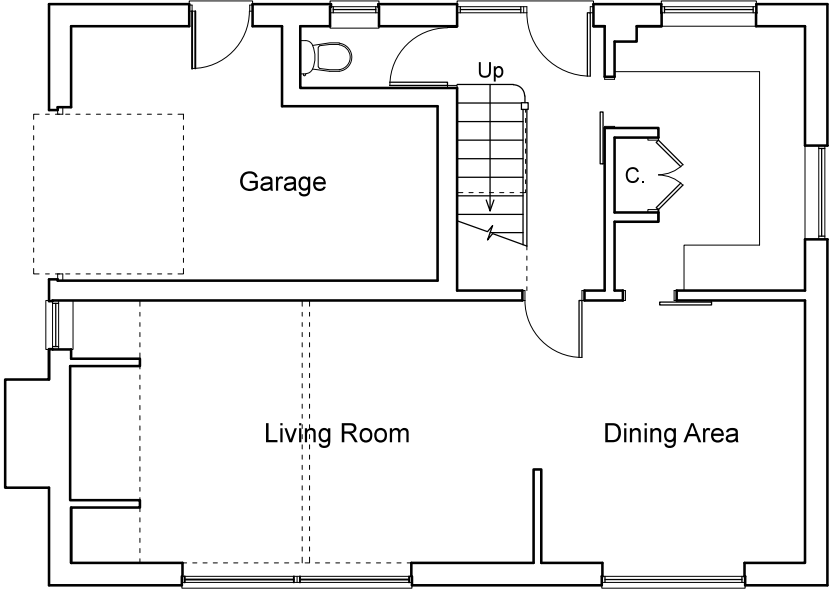
Ground Floor Plan Existing
