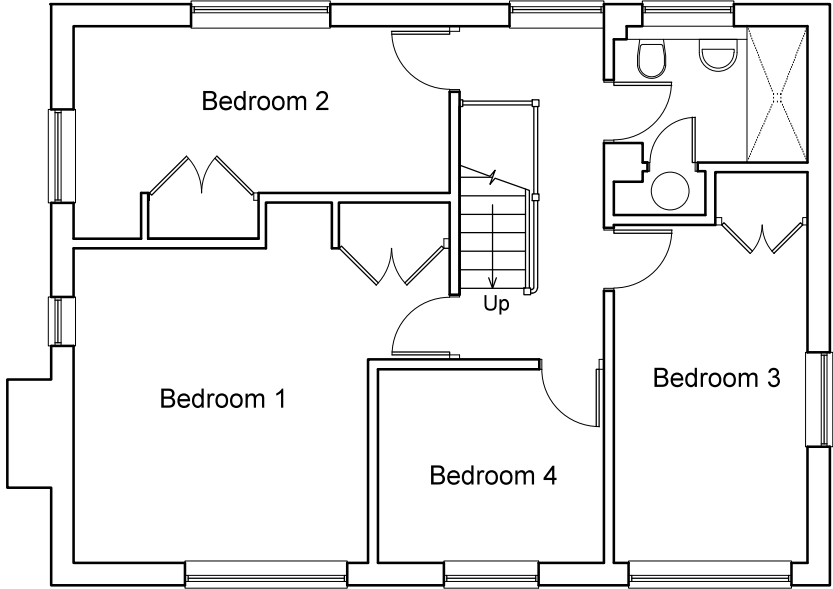
First Floor Plan Existing
