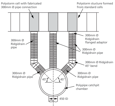
Figure 41 Typical Polystorm 450mm inlet manifold detail
