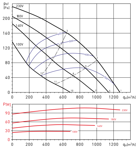
CVAB/4-1400/250N D
