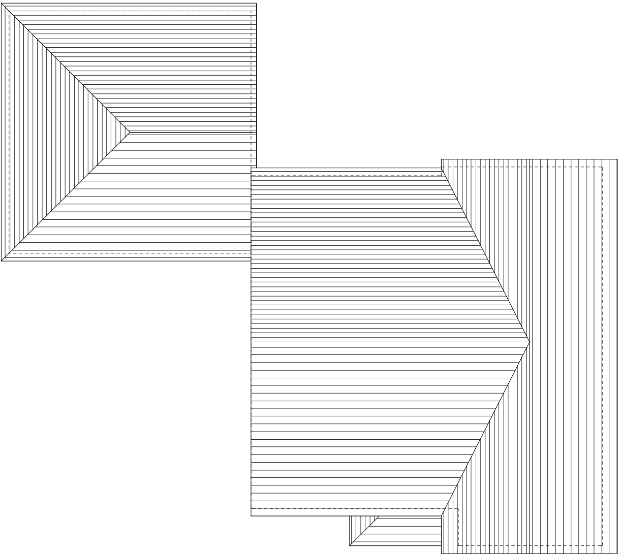
ROOF plan
