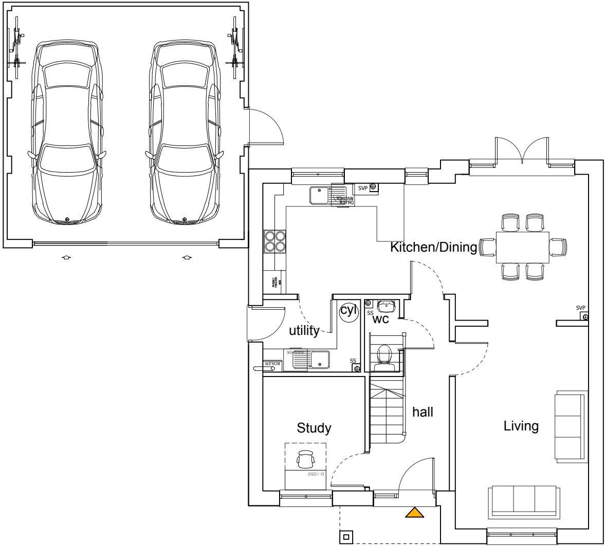
GROUND plan
