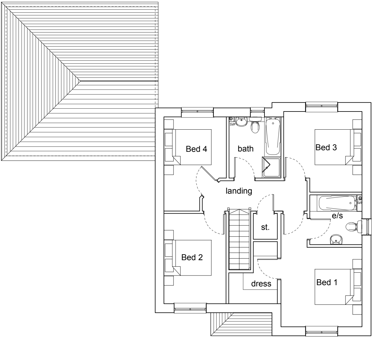
FIRST plan
