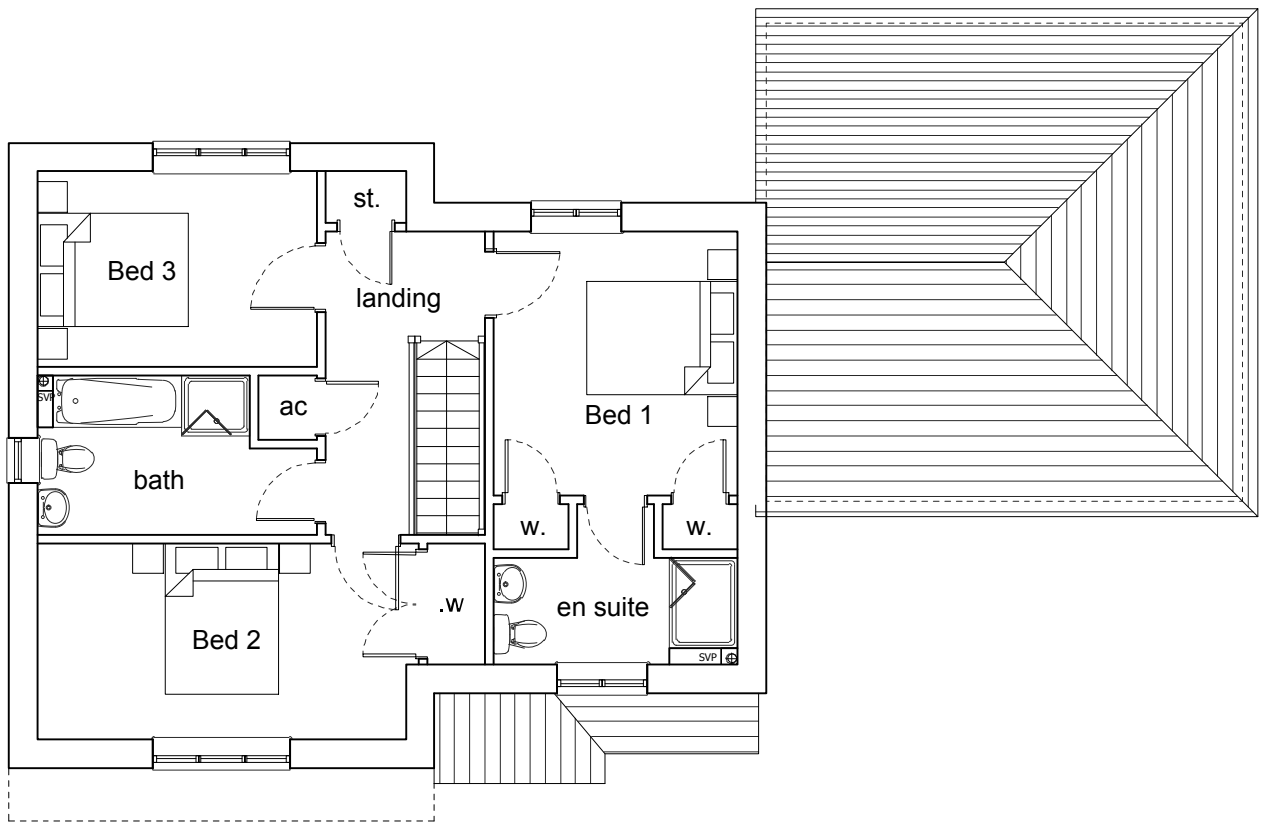
FIRST plan
