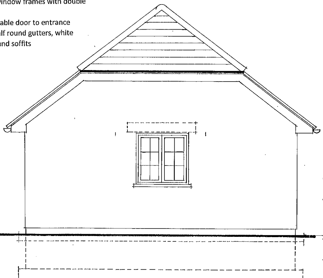
SOUTHWEST ELEVATION TO WEST WALBERTON LANE
