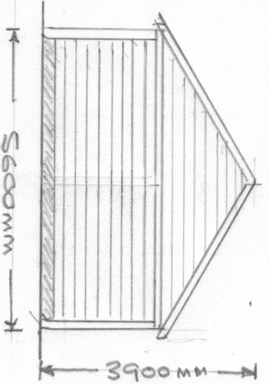
Ⓓ RIGHT SIDE
