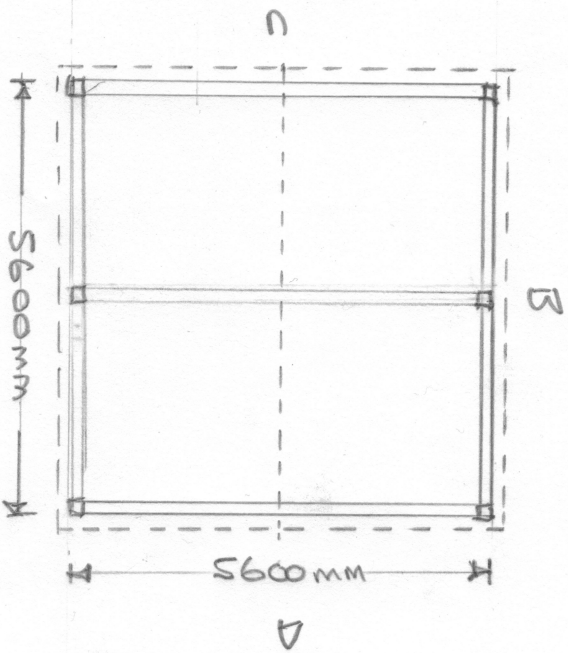
PLAN VIEW
