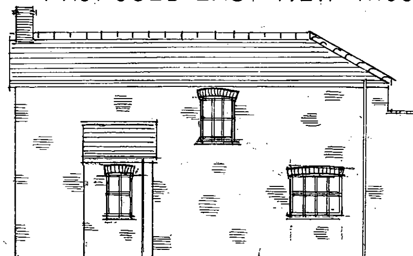
PROPOSED WEST VIEW 1:100
