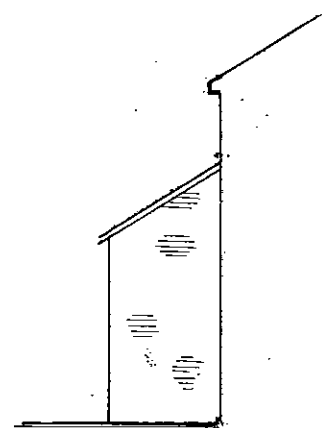
PROPOSED PORCH SOUTH SOUTH VIEW 1:100
