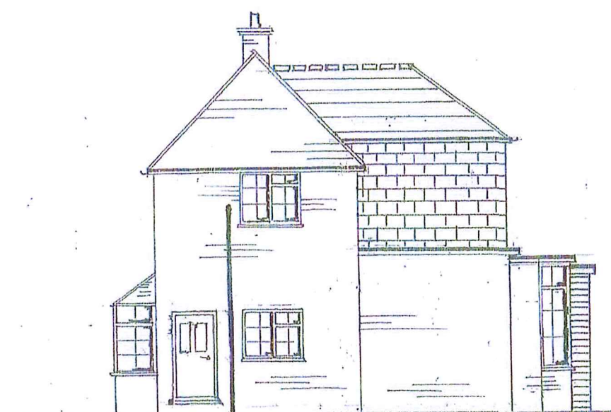
NORTH ELEVATION.
