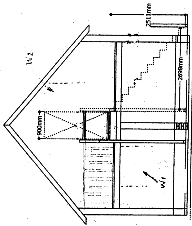
Stair Elevation
