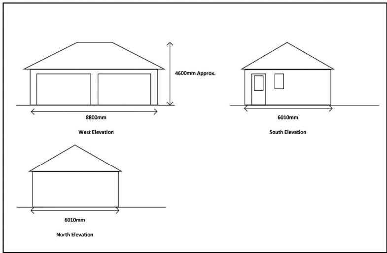
ELEVATION PLAN
