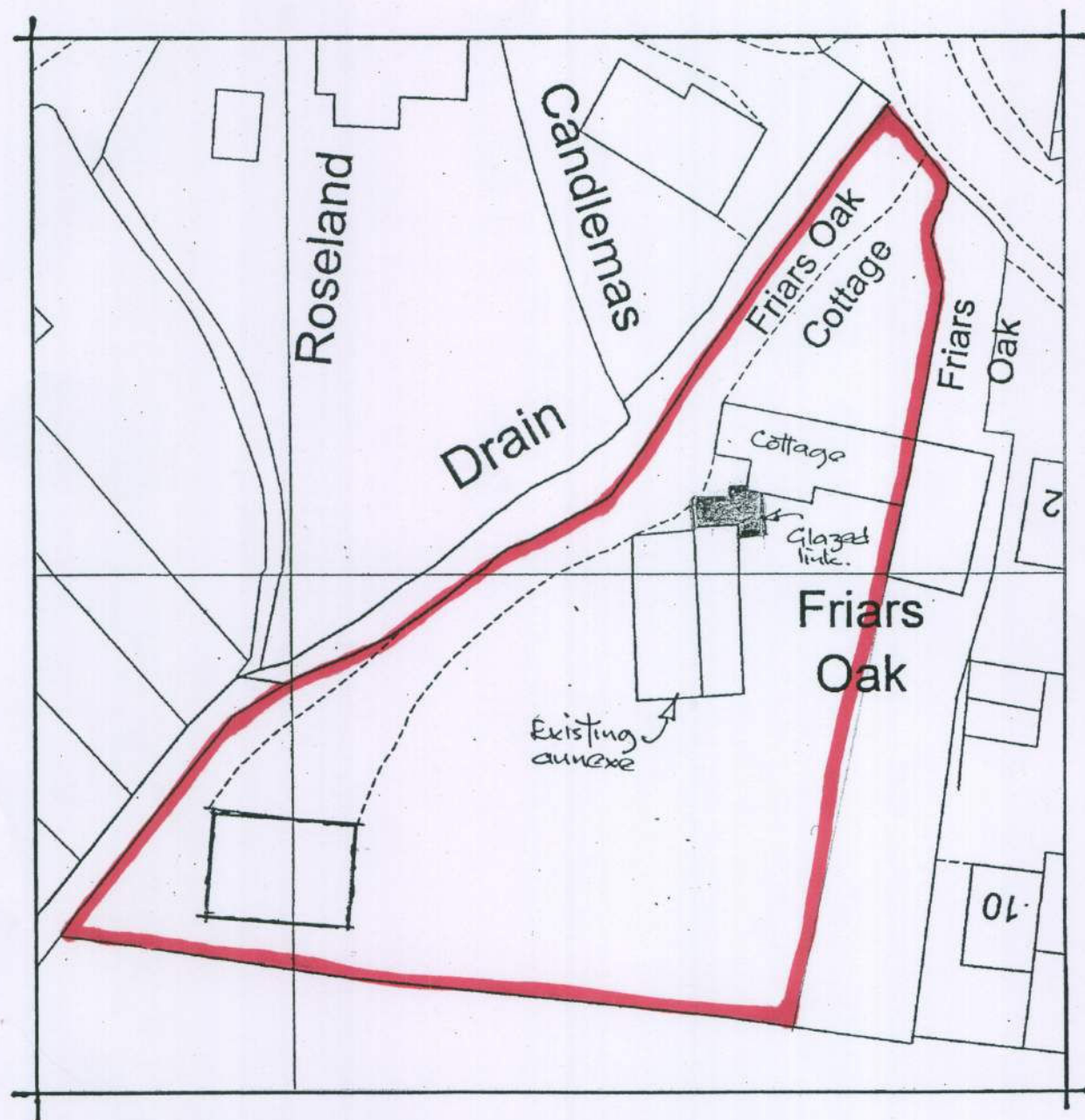
BLOCK PLAN 1:500
