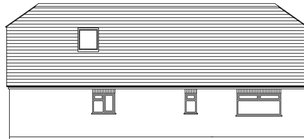
Proposed East Elevation Proposed Neighbour Side Elevation
