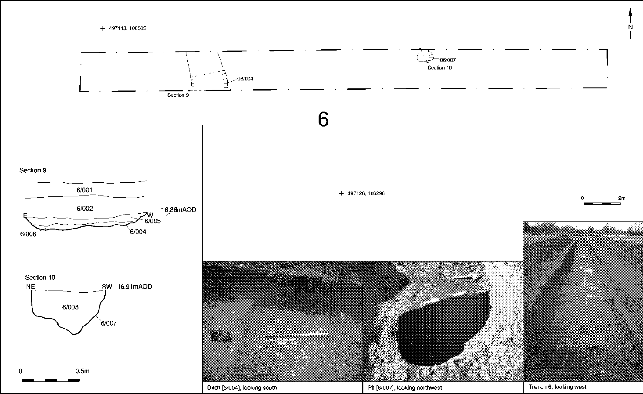
© Archaeology South-East Land East of Tye Lane, Walberton, West Sussex Fig. 9 Project Ref: 180877 February 2019 Trench 6: Plan, sections and photos Report Ref: 2019060 Drawn by: NH
