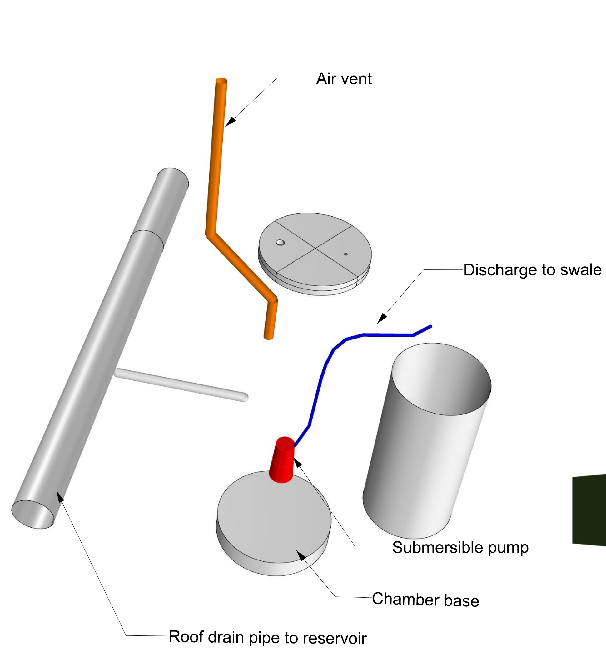
Exploded diagram
