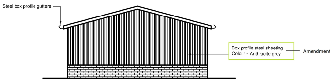
Proposed North East Elevation
