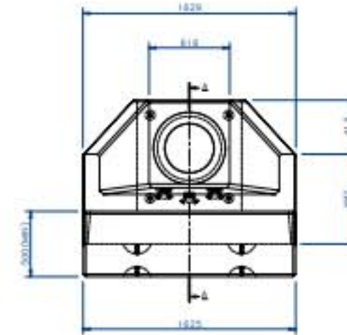
Spillway Headwall S40
