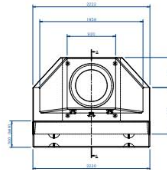
Spillway Headwall S60
