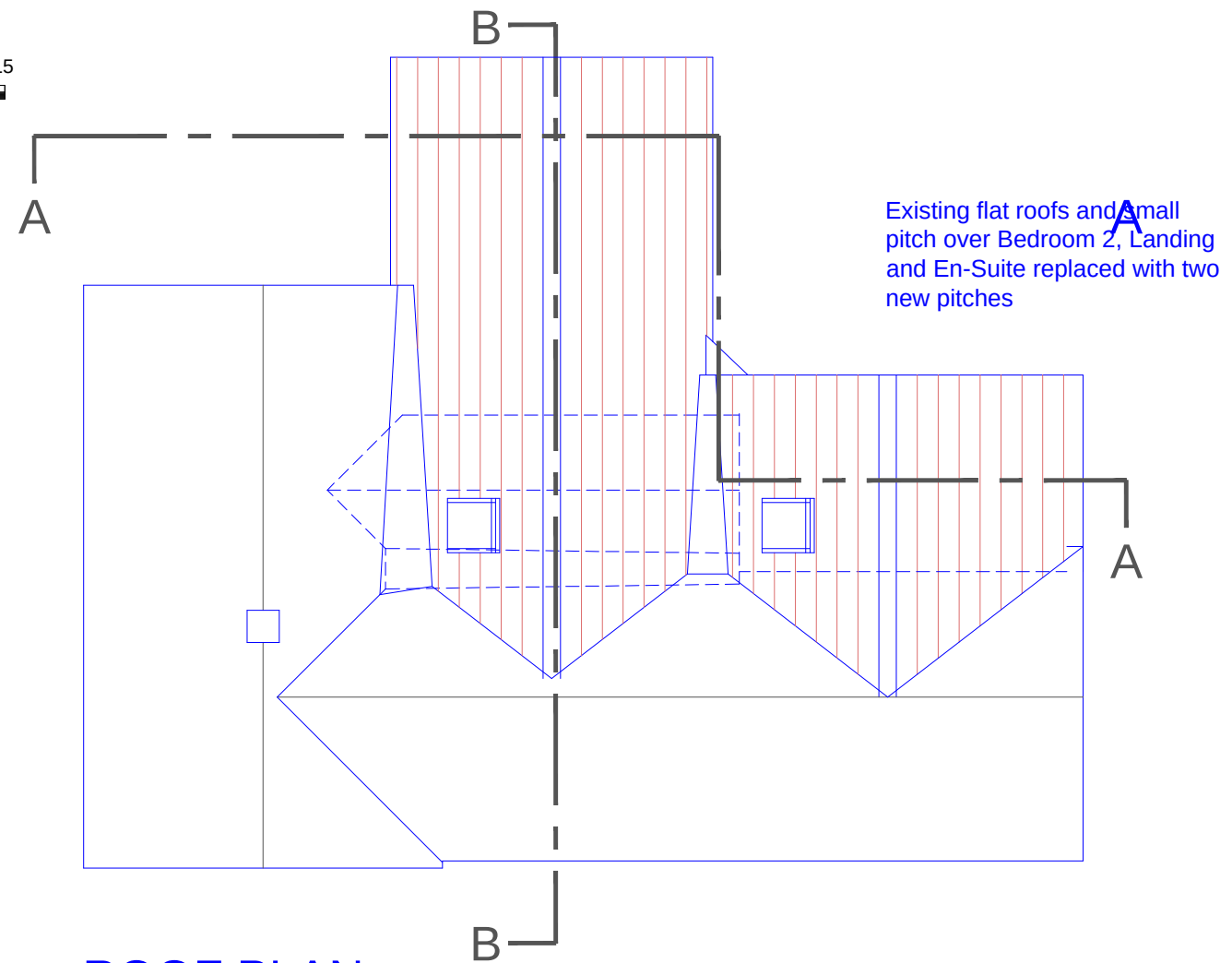
ROOF PLAN Single Storey not shown
