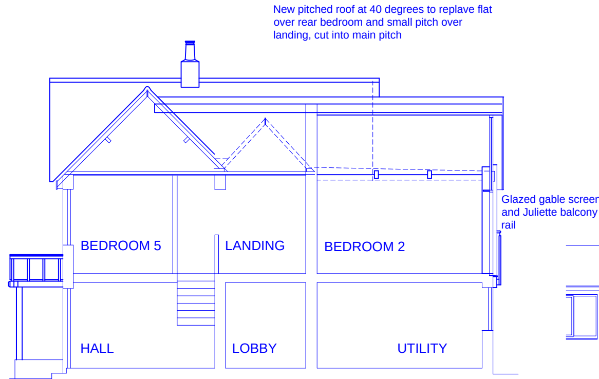
SECTION B
