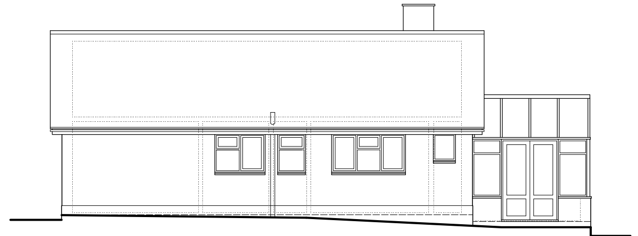
North Elevation
