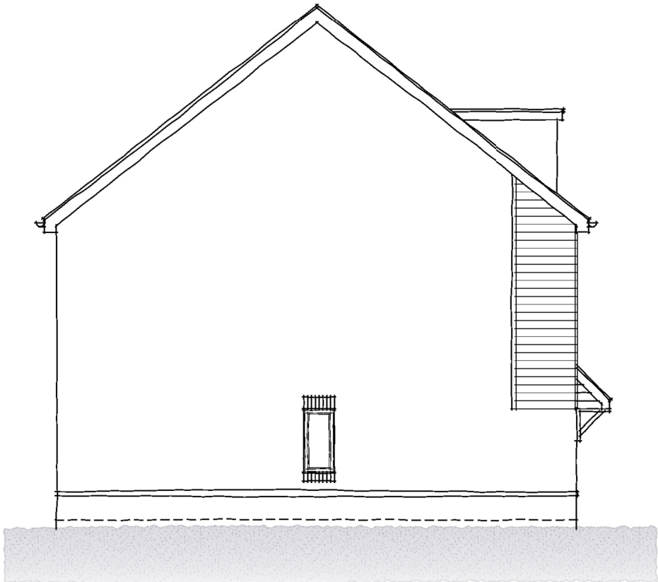
SIDE ELEVATION
